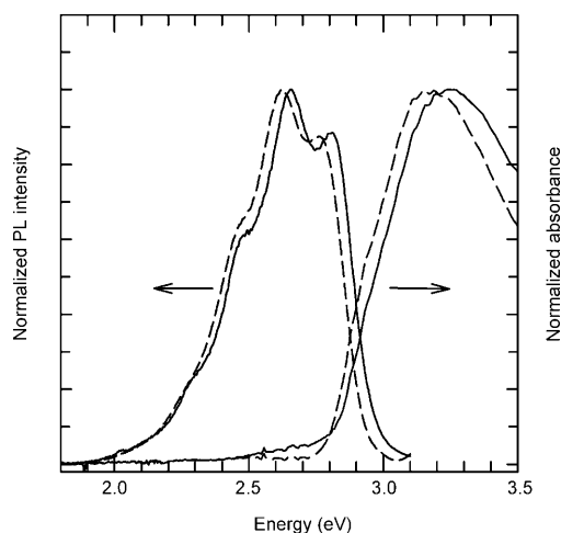
Figure 8. Optical absorption and continuous wave (cw) photoluminescence spectra excited at 3.34 eV for solutions ( 5 \times 10^{-2} mg mL ^{-1} of the conjugated portion) of 1 in \beta -CD and dumbbell 1 in DMSO (—: with \beta -CD, ----: without \beta -CD).
