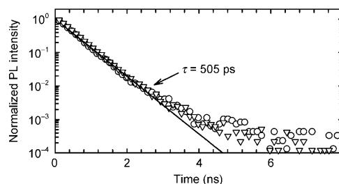
Figure 9. Time-dependent decays of 1 in \beta -CD (circles) and dumbbell 1 (triangles) in DMSO ( 5 \times 10^{-2} mg mL ^{-1} ) excited at 3.3 eV. The PL decays were fitted with a single exponential function, thereby yielding an experimental lifetime \tau = 505 ps. The fitting curve is reported as solid lines ( \circ : with \beta -CD, \nabla : without \beta -CD).
